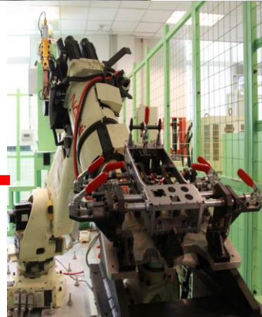
Robotic Welding
